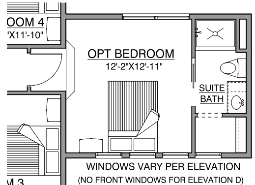
WINDOWS VARY PER ELEVATION (NO FRONT WINDOWS FOR ELEVATION D) OPT. BEDROOM W/ BATHROOM
